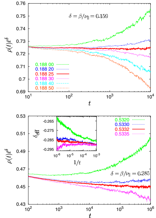
FIG. 1 (color online). Semilog plots of \rho(t)t^\delta vs t for DBAW1 (upper panel) and DBAW2 (lower panel). We use \delta = 0.159 for DBAW1 and 0.285 for DBAW2. Since DBAW2 shows a long-term correction to scaling, we also draw the effective exponents in the inset of the lower panel and find \delta \approx 0.285(1) for DBAW2 which is consistent with the PC value.
