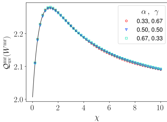
FIG. 1. The TUR factor Q for the molecular refrigerator as a function of the rescaled observation time \chi . Red circles, blue down-triangles, and cyan squares are the numerical results for (\alpha, \gamma) = (0.33, 0.67) , (0.5, 0.5) , and (0.67, 0.33) , respectively. For this calculation, m = 1 and T = 1 are used. The black solid curve denotes the analytic result (27).
